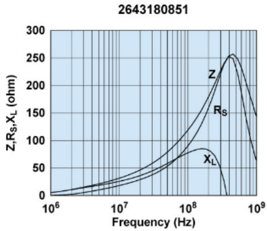
Impedance, reactance, and resistance vs. frequency.
